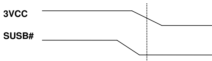
Figure 14.4 The previous state is "off" - 3VCC falls to 2.6V and SUSB# keeps at 0.8V
