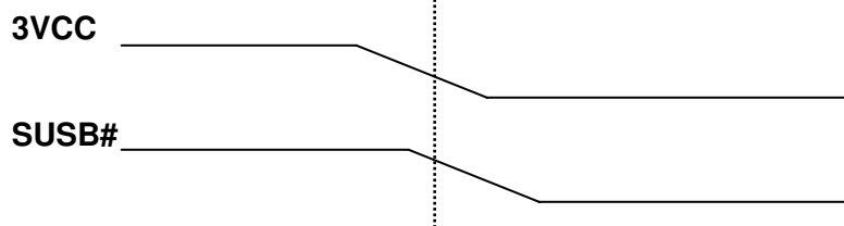
Figure 14.3 The previous state is "on" - 3VCC falls to 2.6V and SUSB# keeps at 2.0V
